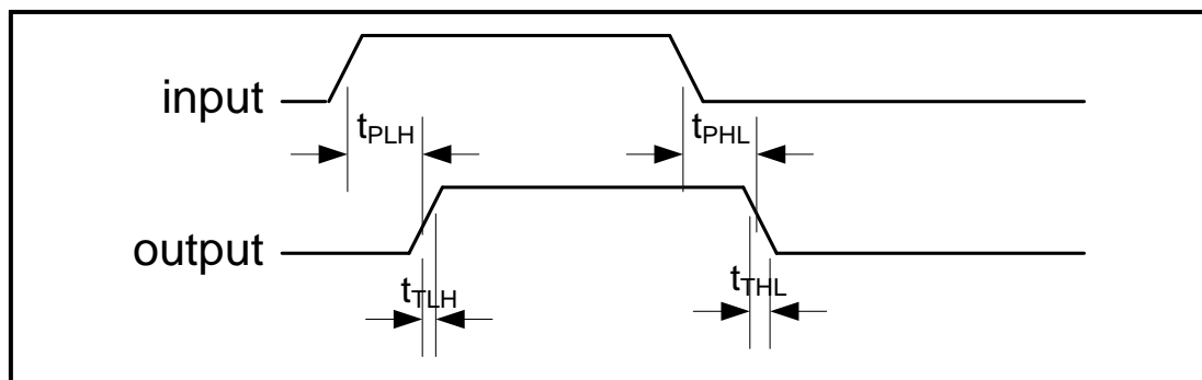
Figure 2. AC Waveforms
