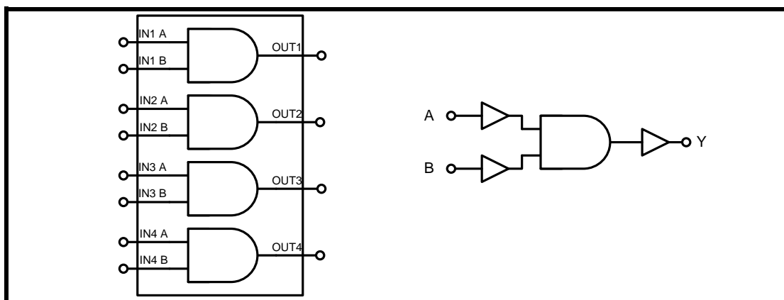
Figure 1. CHT-7408: simplified block diagram.
