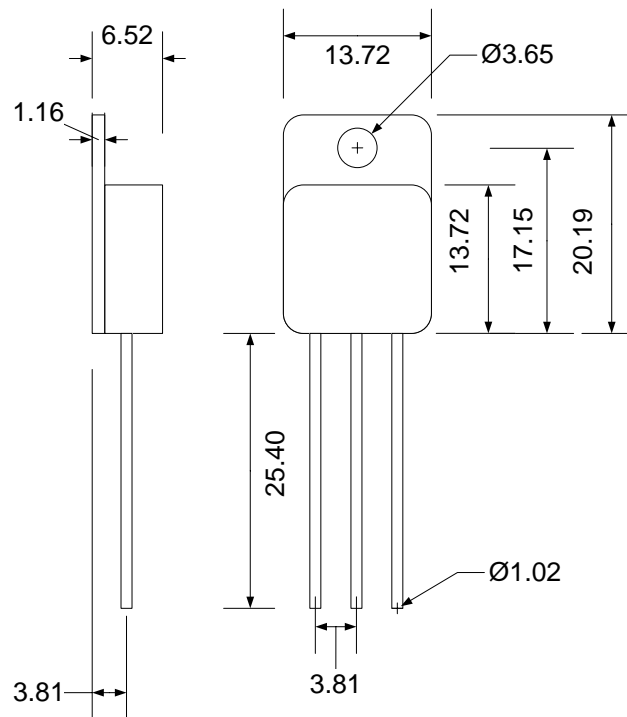
TO254 (mm +/- 10%)
