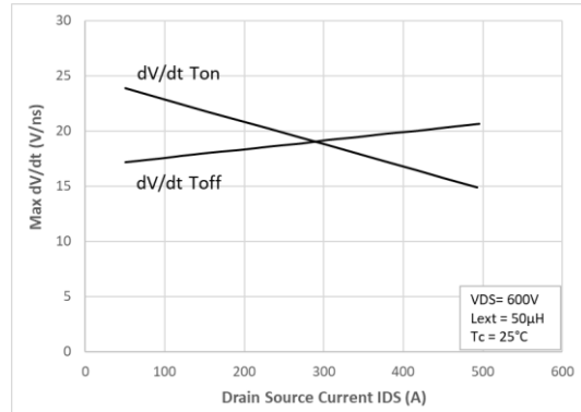
Figure 12 : Max dV/dt vs Drain current
