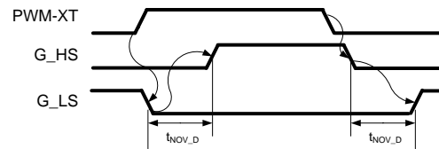
Figure 21: Local Mode operation
