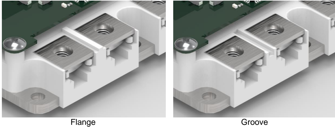
Figure 26: DC power terminals separation solutions
