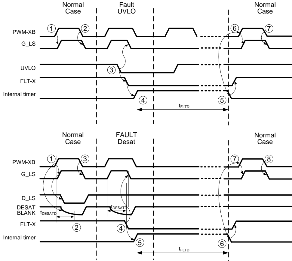
Figure 25: Timing diagram CXT-PLA3SA12340A low-side gate driver behaviour
